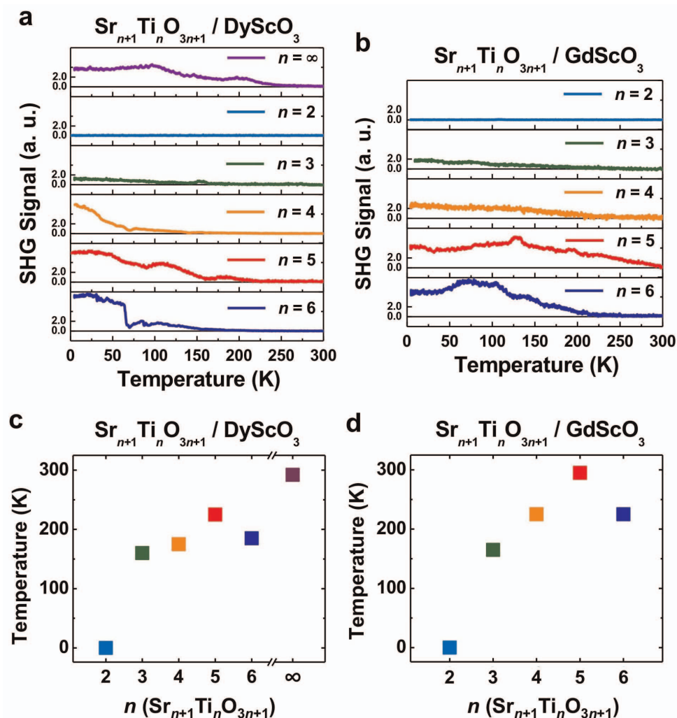
Extended Data Figure 5 | Nonlinear optical SHG temperature scans of \text{Sr}_{n+1}\text{Ti}_n\text{O}_{3n+1} ( n = 2 – 6 and n = \infty ) films. a , Films grown on (110) \text{DyScO}_3 . b , Films grown on (110) \text{GdScO}_3 substrates. The SHG signal for each temperature scan was normalized with the laser input power, where the SHG signal axis for each scan shows normalized tick labels at 0 and 2 to compare the
