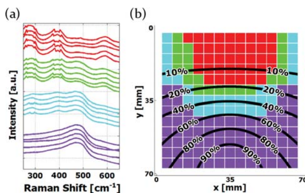
Figure 4. Hierarchical clustering analysis of the Raman data: (a) Five random spectra chosen from each of the four groups, demonstrating similarity between spectra within the same group, and the dissimilarity between spectra from different groups. (b) The four groups of similar Raman spectra marked on the library map by different colors. The composition (Nb percentage) is indicated by black contours. It is clear that some of the points with similar composition have very different Raman spectra.
