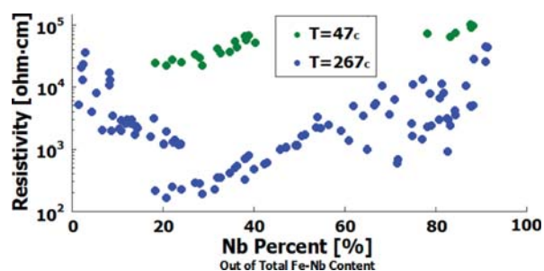
Figure 3. Resistivity [ \rho ] as a function of the Nb percentage (out of the total Fe–Nb content in the Fe–Nb–O layer), measured at 47 °C [green] and at 267 °C [blue]. A large fraction of the library was too resistive to measure at the former temperature. To circumvent this restriction, the sample temperature was raised to decrease the resistivity in accordance with fundamental semiconductor theory. Even in the high temperature (267 °C), only 103 of the 169 points of the library were successfully measured, while 66 points were still too resistive for measurement, mainly at points with close to pure \text{Fe}_2\text{O}_3 (far left of the plot) and \text{Nb}_2\text{O}_5 (far right of the plot). In the blue graph (267 °C), some mixing ratios of Nb show a significant difference in resistivity (more than an order of magnitude) for the same Nb percentages. This phenomenon is especially evident at the two minimum points; with discontinuity at \sim 20\% Nb and scattered results at \sim 70\% Nb. The same two minimum points are also observed in lower temperature (47 °C), as can be seen in the green plot.
